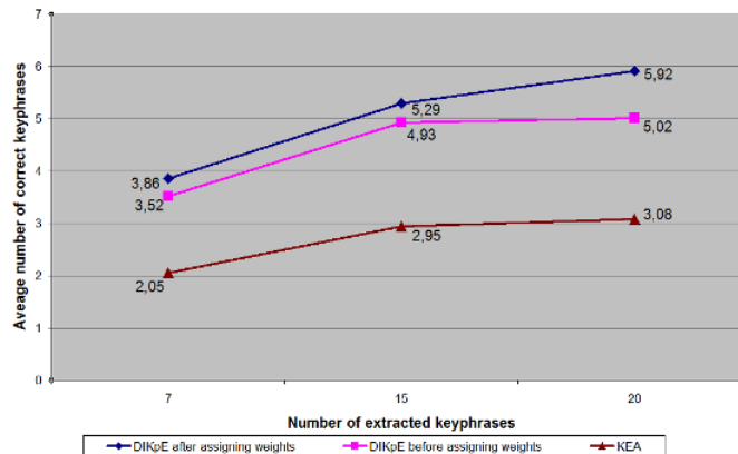
Figure 5. Performance of DIKpE compared to KEA
