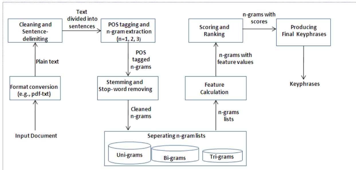
Figure 2. Workflow in DIKpE system
